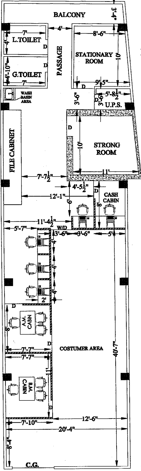
FIRST FLOOR
