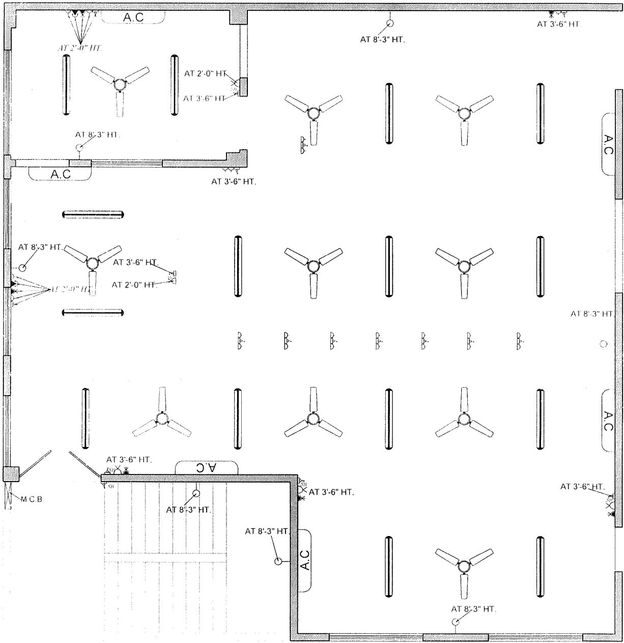
FIRST FLOOR BANK INTERIOR LAYOUT
